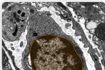
Nuclei (TEM)
